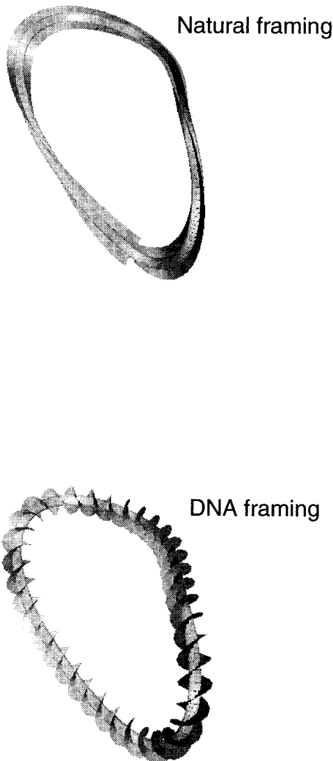
FIGURE 2 Natural and DNA framings of a ring equilibrium. The two framings are related through the known DNA-frame intrinsic twist (see text). Note that a cyclized DNA frame as shown here will not in general correspond to a cyclized natural frame.
